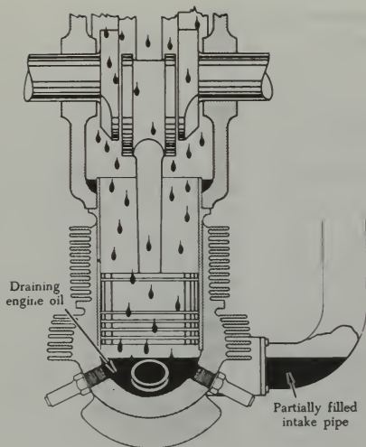
FIGURE 10-44. Initial step in developing a hydraulic lock.
